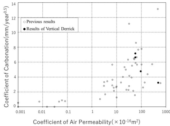
Figure 7. Relation between coefficient of air permeability and coefficient of carbonation. (Akio Tanaka; Kei-ichi Imamoto, 2013)
