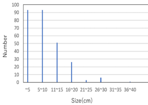
Figure 5. Size of concrete flakes.
