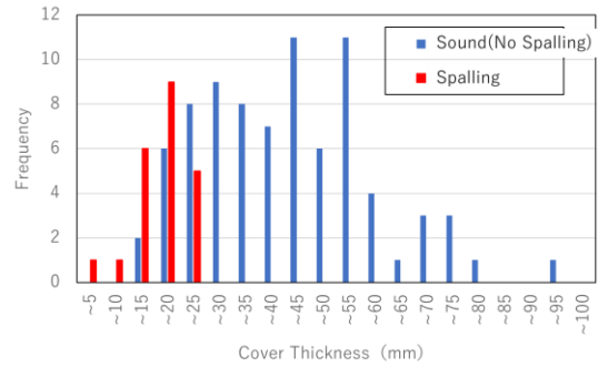
Figure 6. Cover thickness and rebar expose. (Tomotaka Ide, 2019)
