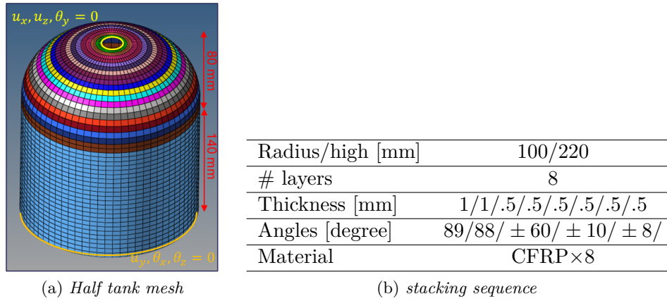
Figure 8: Half tank
