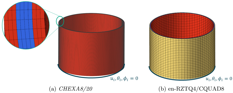
Figure 5: Cylinder mesh
