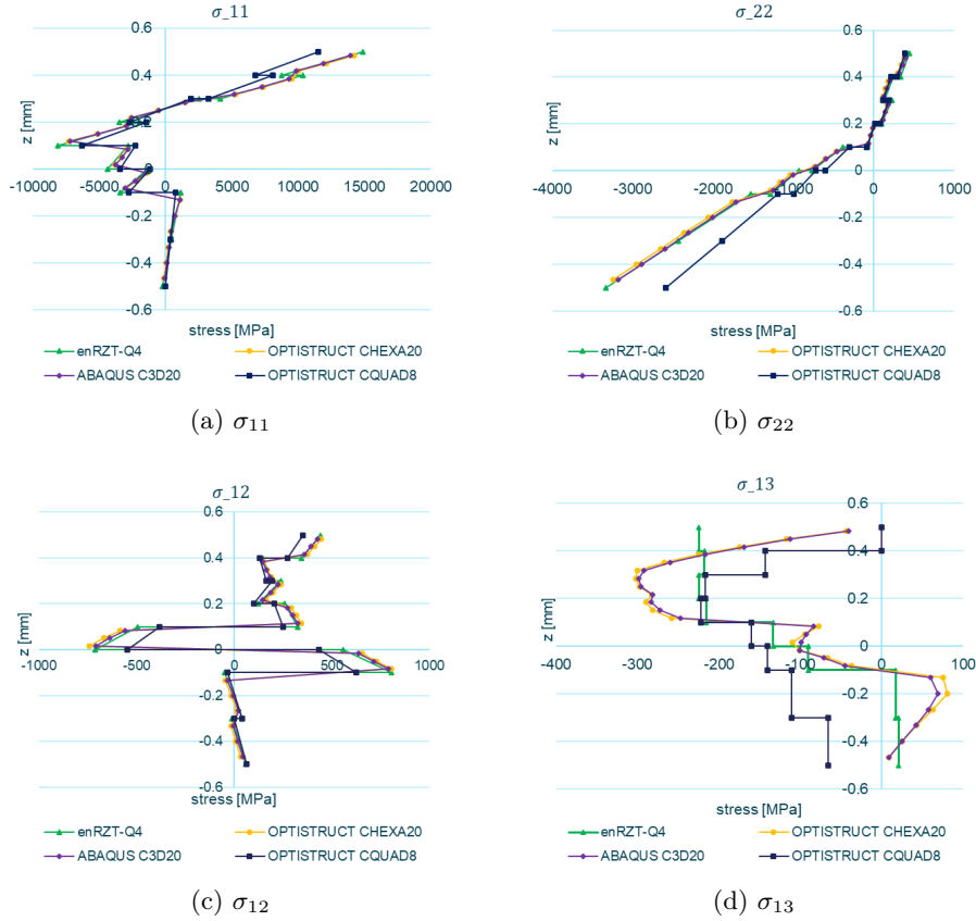
Figure 11: Cantilivered plate stresses
