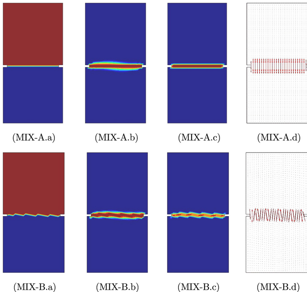
Fig. 10. Results for rectangular strip under tension using the mixed formulation and triangular meshes (top: mesh A, bottom: mesh B). Contours of: (a) total displacement, (b) damage index (c) major principal strain. (d) Vectors of major principal strain.
