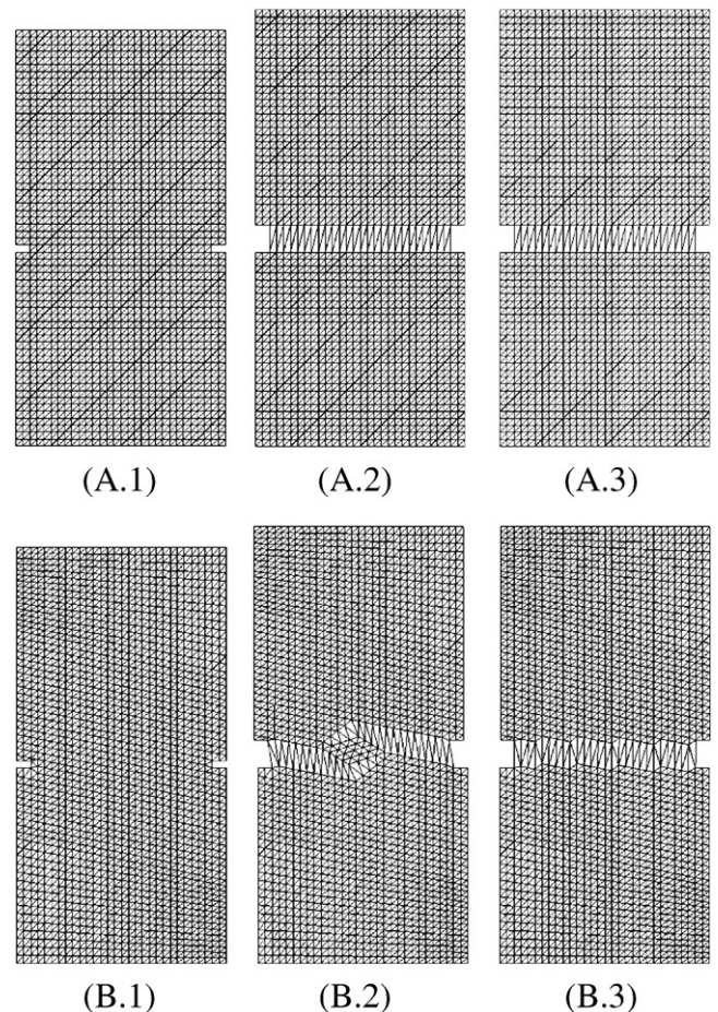
Fig. 7. Triangular meshes A and B for the rectangular strip under tension: (1) undeformed shape, (2) deformed shape – irreducible form, (3) deformed shape – stabilized mixed form.
