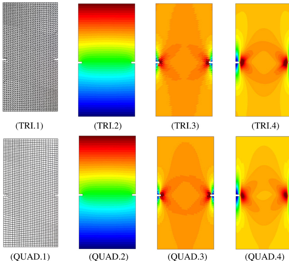
Fig. 3. Results for rectangular strip under tension (top: triangular mesh, bottom: quadrilateral mesh). Contours of: (2) total displacement, (3) major principal strain – irreducible form, (4) major principal strain – stab. mixed form.
