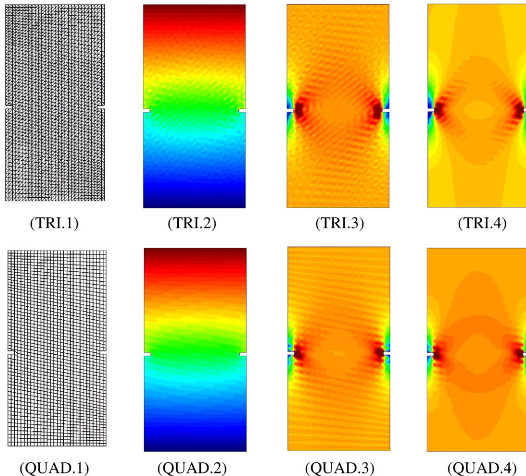
Fig. 4. Results for rectangular strip under tension with the mixed formulation (top: triangular mesh, bottom: quadrilateral mesh). Contours of: (2) total displacement – no stabilization, (3) major principal strain – no stabilization, (4) major principal strain – strain stabilization only.
