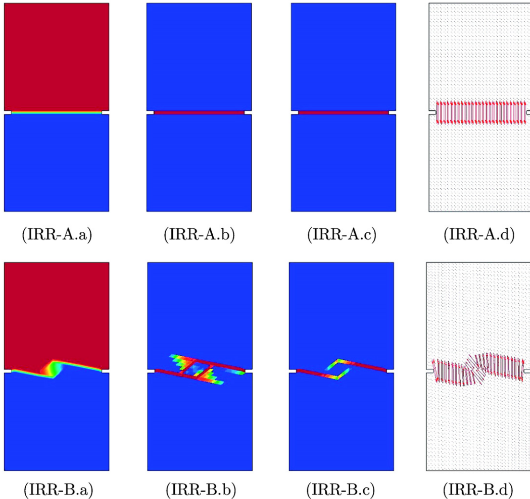
Fig. 9. Results for rectangular strip under tension using the irreducible formulation and triangular meshes (top: mesh A, bottom: mesh B). Contours of: (a) total displacement, (b) damage index (c) major principal strain. (d) Vectors of major principal strain.
