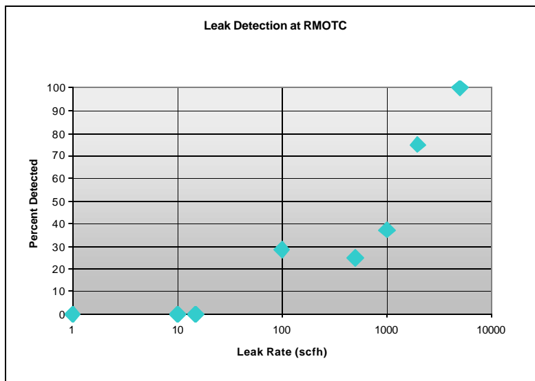
Figure 22. ANGEL System leak detection summary for RMOTC Field Test, Sept. 14-17
