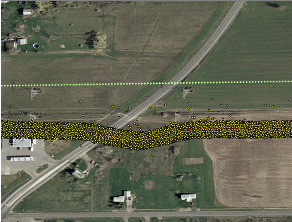
Figure 13. A geo-referenced color image of the pipeline right-of-way is used as a base GIS raster imagery layer. The GIS vector layer of the pipeline supplied by National Fuel is indicated in red, the track of the ANGEL system aircraft as it flew the line is marked in green. Yellow dots indicate the position of individual laser spots along the inspection swath of the DIAL system.
