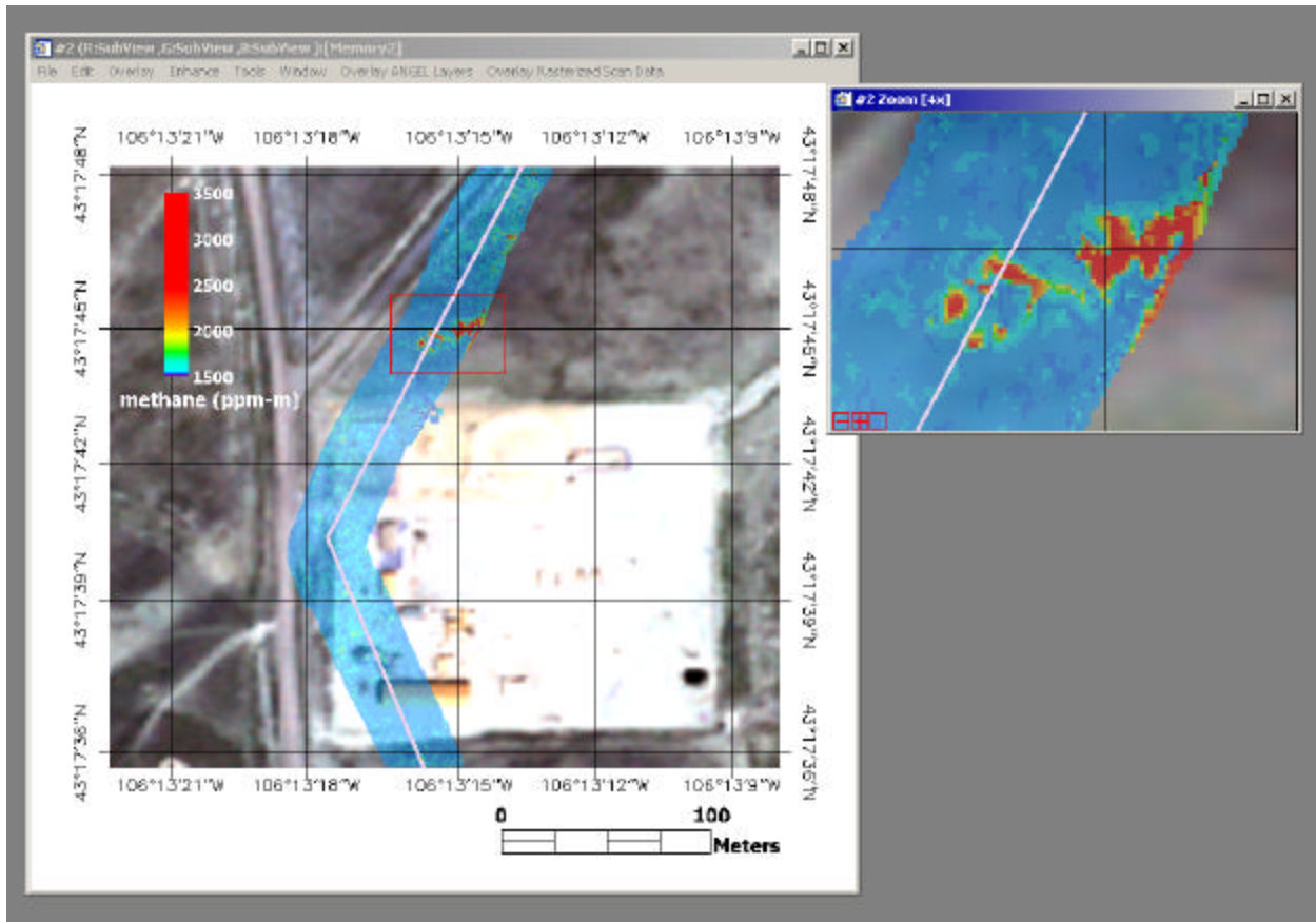
Figure 10 Detection, quantification, visualization, and geolocation of a natural gas plume at RMO TC.
