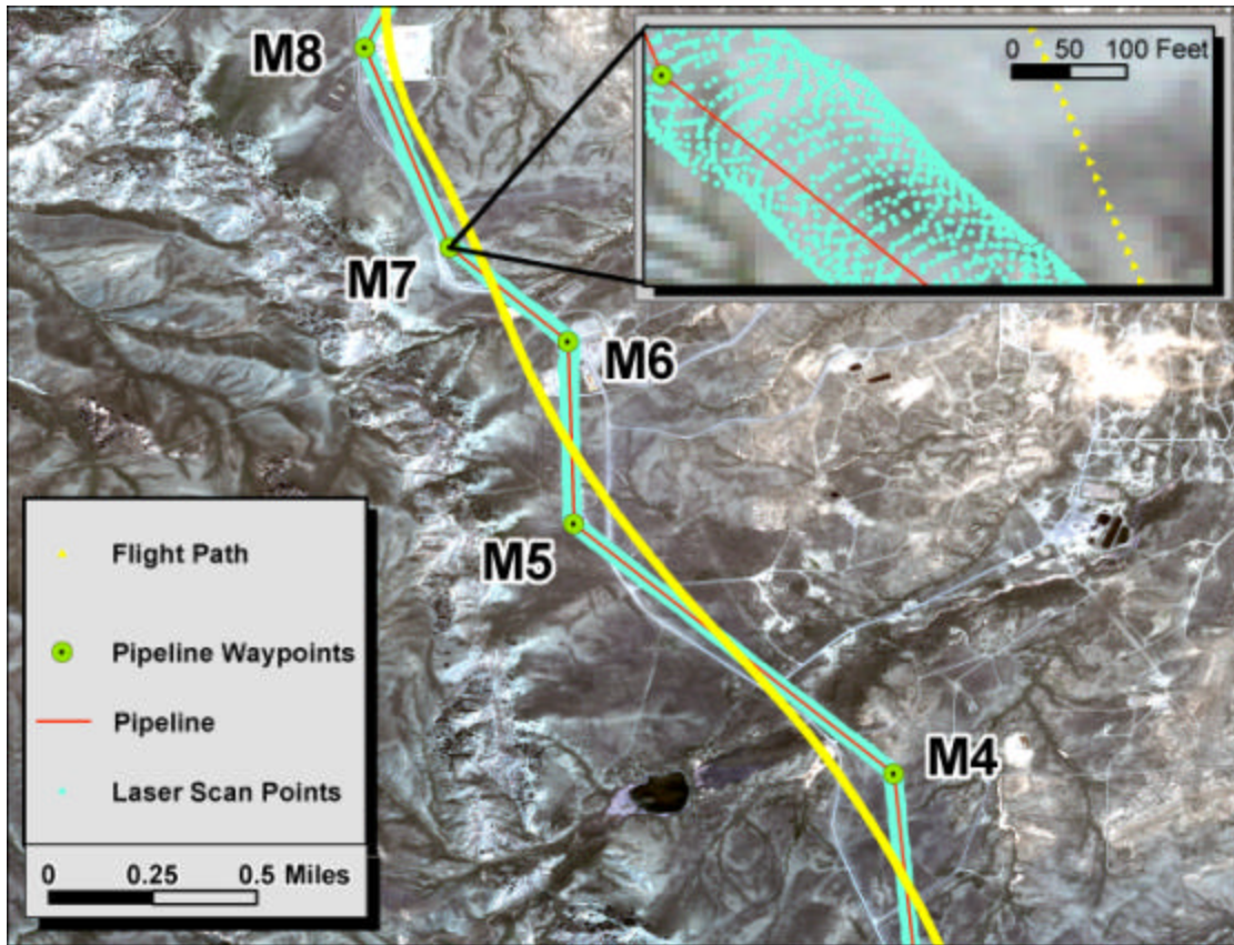
Figure 5 Space Systems ANGEL pointing results from a short section of the Virtual Pipeline Route at RMOTC. The aircraft path is shown in yellow. The pipeline position is shown in red. The position of each data point is shown in green forming a coverage swath 110 feet wide. The sensor pointing and scanning system allows full coverage of the ROW corridor in a single pass.
