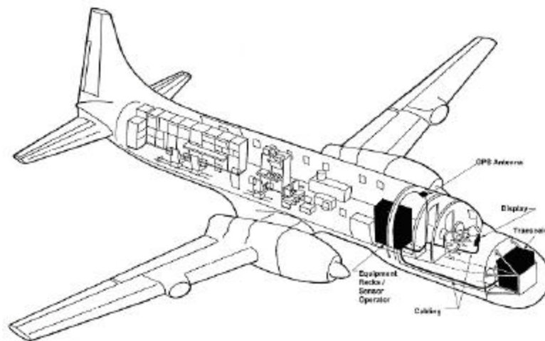
Figure 7. Diagram of Space Systems ANGEL System Test Aircraft illustrating placement of the major sensor components.
