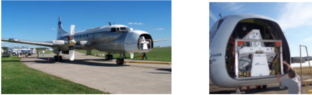
Figure 8. Space Systems ANGEL System Test Aircraft showing placement of the transceiver in the nose of the aircraft during preparation for early flight tests in Buffalo, NY.
