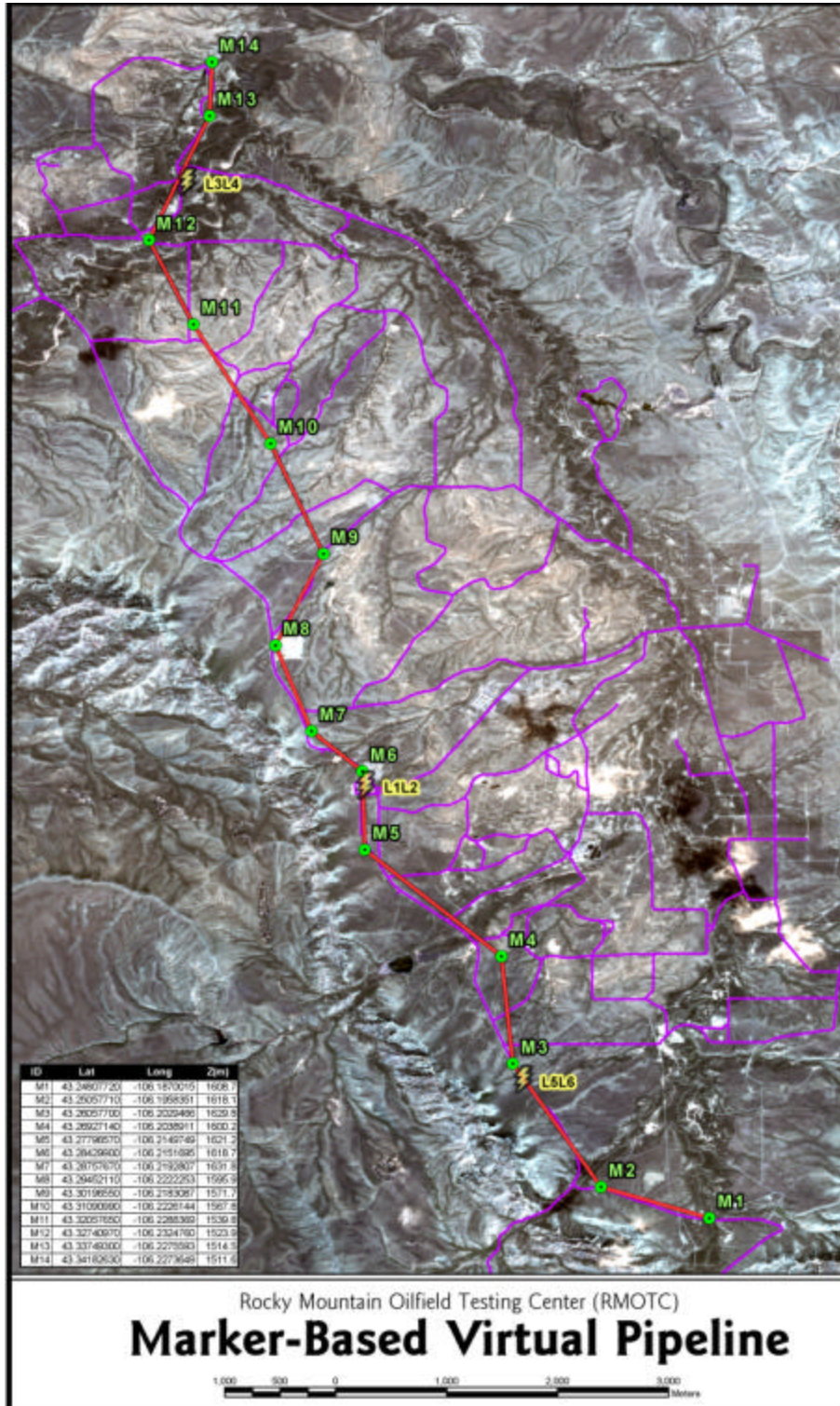
Figure 18. Map of the Marker-Based Virtual Pipeline along the western edge of the Rocky Mountain Oilfield Testing Center in Wyoming. Virtual pipeline in shown in Red, 14 pipeline markers of known location are shown in green, meteorology stations are shown in yellow.
