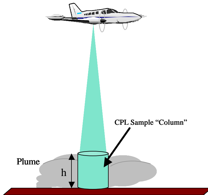
Figure 3. Concentration Path Length (CPL) of a plume as measured from an aircraft.
