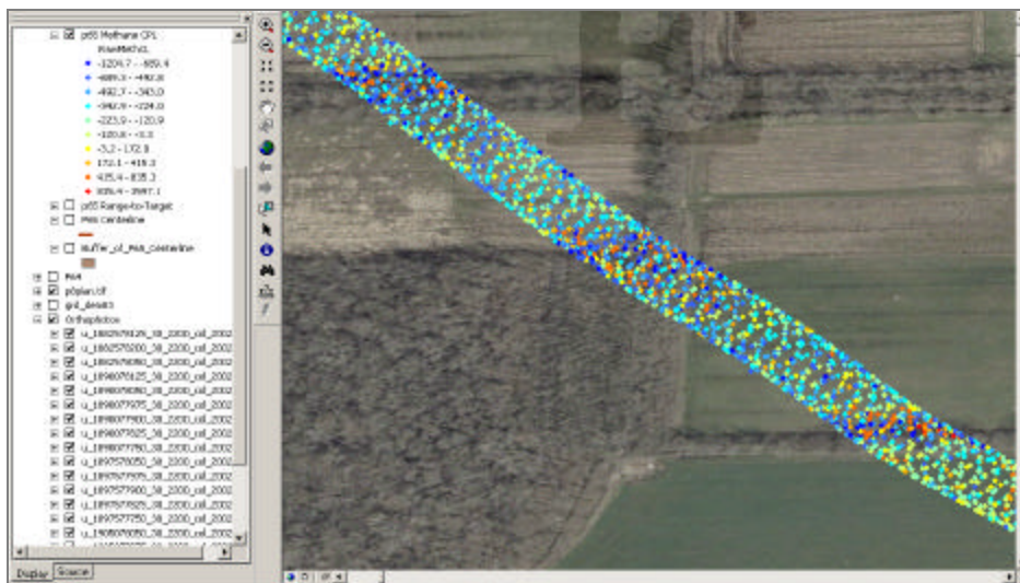
Figure 15. First airborne DIAL data set from the ANGEL sensor processed color-coded for methane concentration path length (CPL). Methane CPL in this “first light” image are highly variable and greatly effected by vegetation. A variety of hardware and software have been implemented to improve the quality the ANGEL data.
