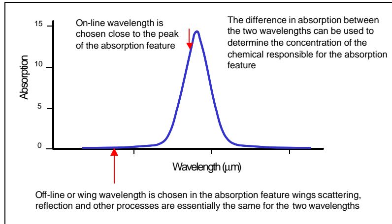
Figure 1. Generic representation of DIAL on-line and off-line positions
