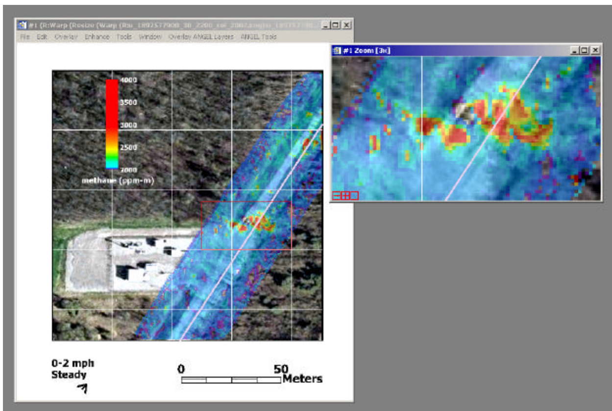
Figure 23. ANGEL DIAL system image of a gas plume from a 3,500 scfh methane release along a tree-lined pipeline right-of-way near Buffalo, NY. This data was in October, 2004 from the TIFS test aircraft flying at 150 mph from a height of 1,000 feet above the ground. This simulated leak was created in cooperation with National Fuel near the Pendleton Meter Station.
