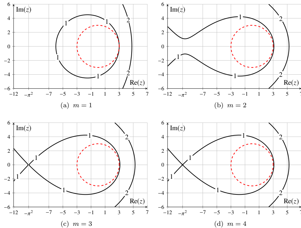
FIG. 4.1. The contours of |w - 1|/2 , where w = r_m(z) is the [m/m] Padé approximant to \cosh \sqrt{z} of degree m \in \{1, 2, 3, 4\} , along with the circle |z| = 3 (dashed line).
