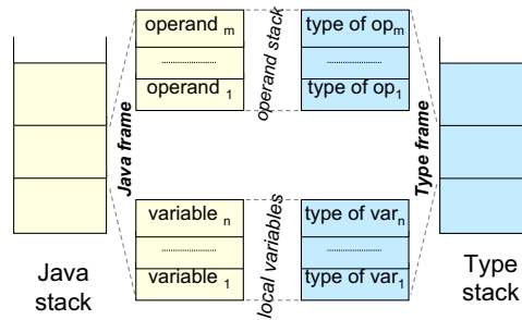
Figure 6: Type stack vs. Java stack
