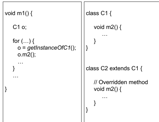
Figure 8: Method inlining and dynamic class loading
