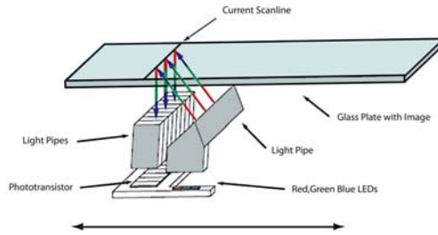
Fig. 2. Contact Image Sensor schematic plan
