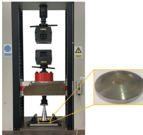
Figure 14: The quasi-static compression test equipment
