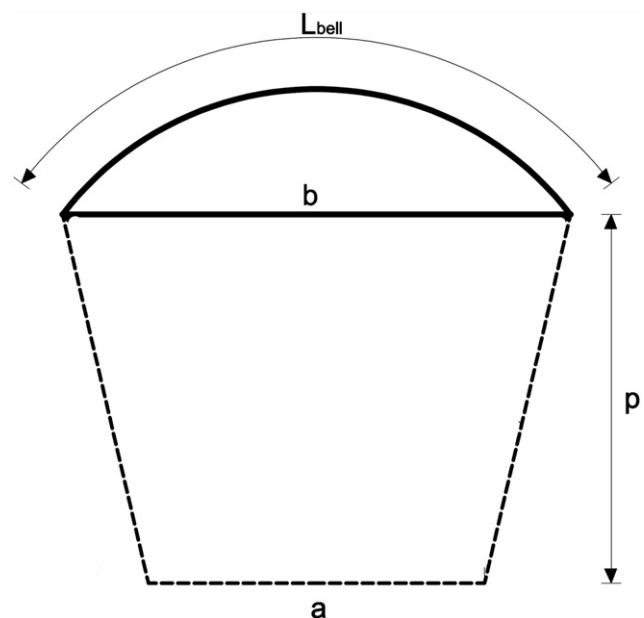
Fig. 1 – Geometrical parameters for the tubular low-cost digester installed in a trench.
