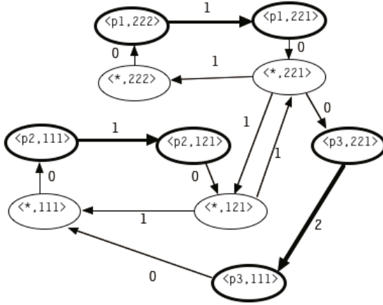
Fig. 9. Example TestEnvGraph
