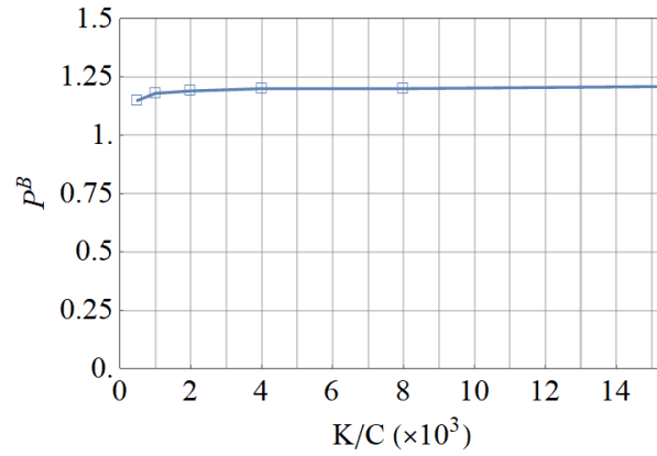
Figure 13: Static bifurcation load for several values of K/C ( \xi=0 ).
