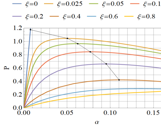
Figure 3: Static equilibrium path P versus \alpha for different imperfection amplitudes \xi .
