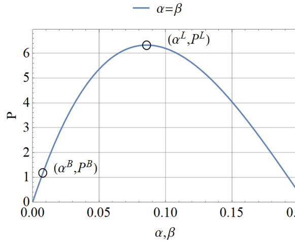
Figure 2: Fundamental static equilibrium path obtained in this work, showing a bifurcation and a limit point.
