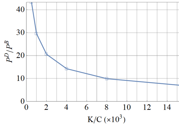
Figure 14: Dynamic quasi-bifurcation load for several values of K/C (assuming that t_0=0.05 , and \xi=0 ).
