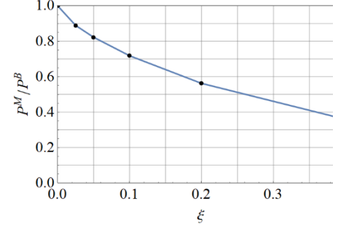
Figure 4: Imperfection-sensitivity under static load.
