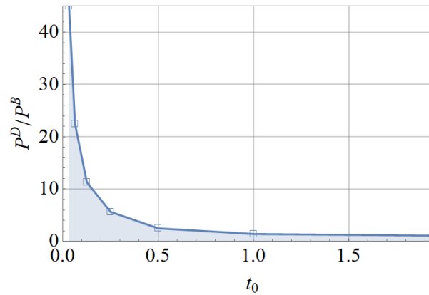
Figure 12: Dynamic quasi-bifurcation load for several values of positive phase duration t_0 of an impulse, assuming perfect system.
