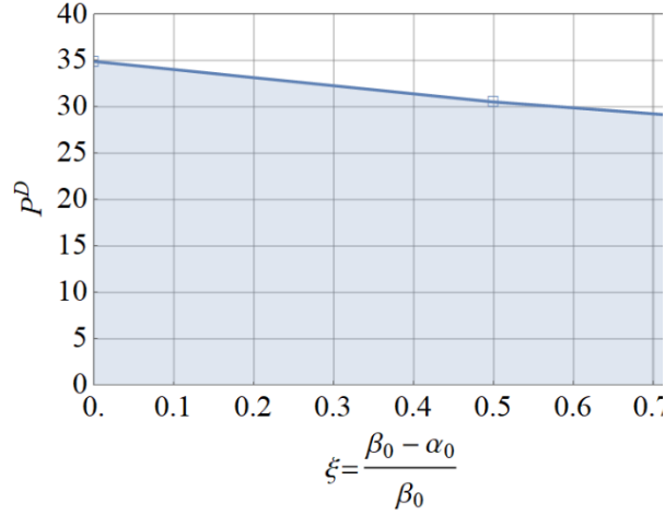
Figure 11: Imperfection-sensitivity curve for dynamic quasi-bifurcation.
