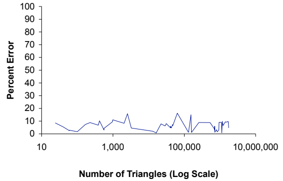
Figure 6: Percentage error of predicted time for the isosurface extraction. Data for graph collected from all machines on which the isosurfacers modeling tests were run.
