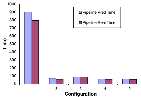
Figure 9: The predicted and real times for visualization pipeline.
